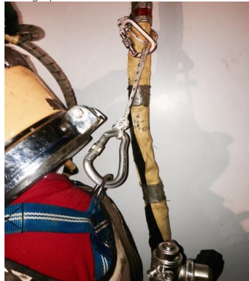
Rescue lanyard used to align IP to trunk
