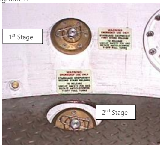
1 st & 2 nd stage release with divers umbilical removed Note: Different bell designs have different layouts
